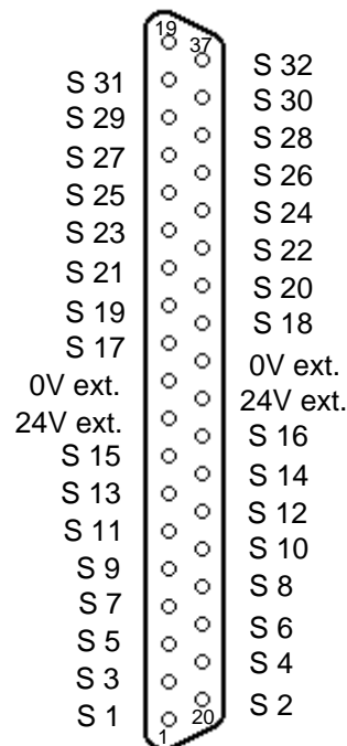
SUB-D37
